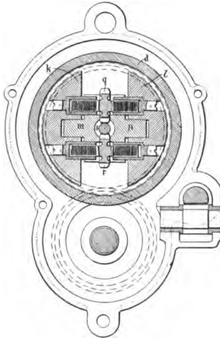
FIG. 358.—Cross Section through the De Dion & Bouton Two-speed Change Speed Gear.
